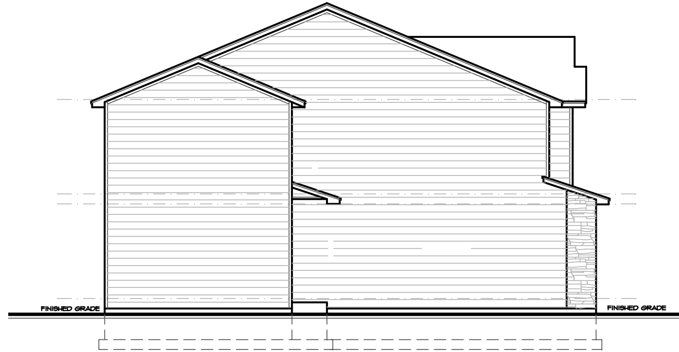
LEFT ELEVATION
