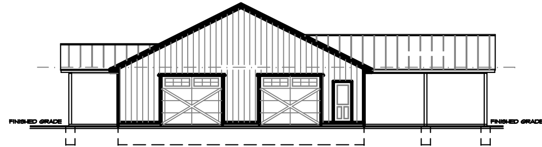
RIGHT ELEVATION SCALE 1/8" = 1'-0"
