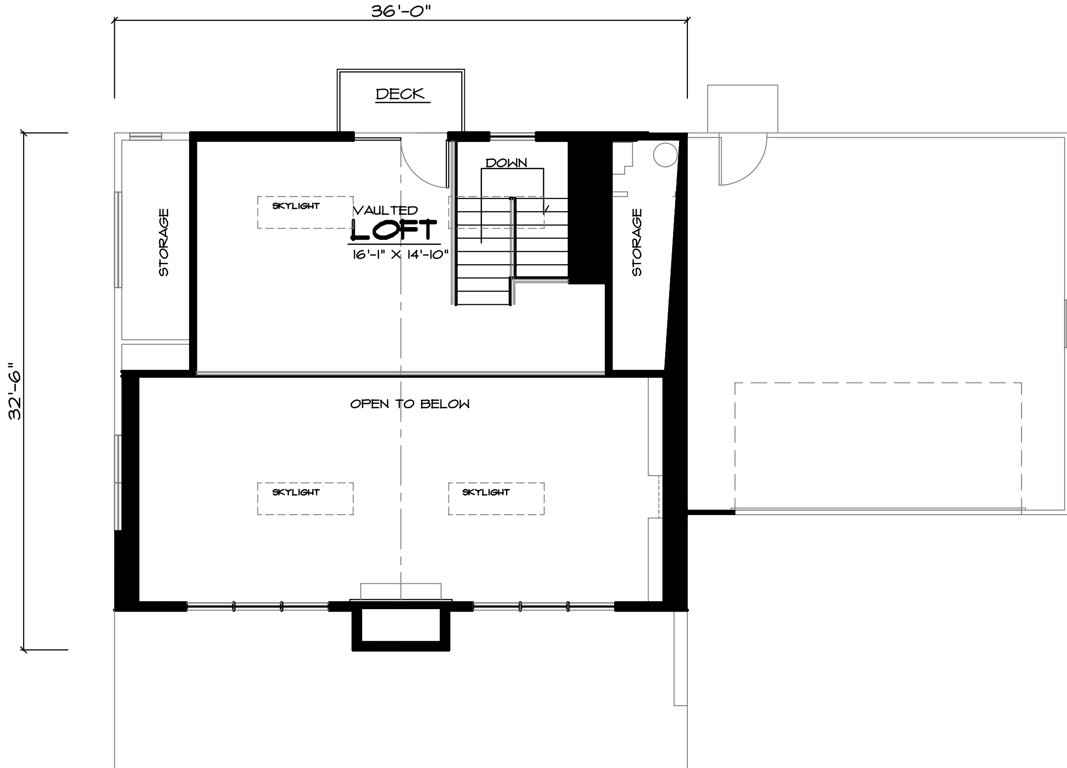
UPPER FLOOR PLAN SCALE 384 SQ. FT. UPPER NTS
