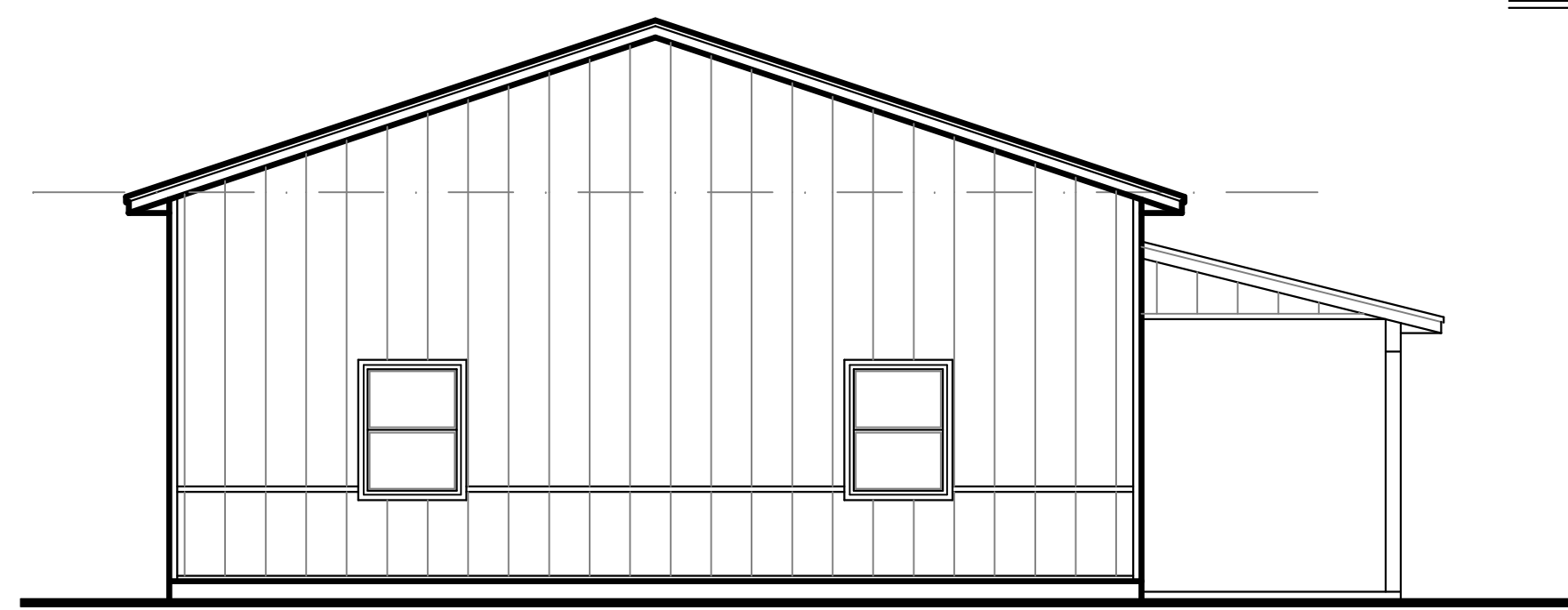
LEFT ELEVATION
