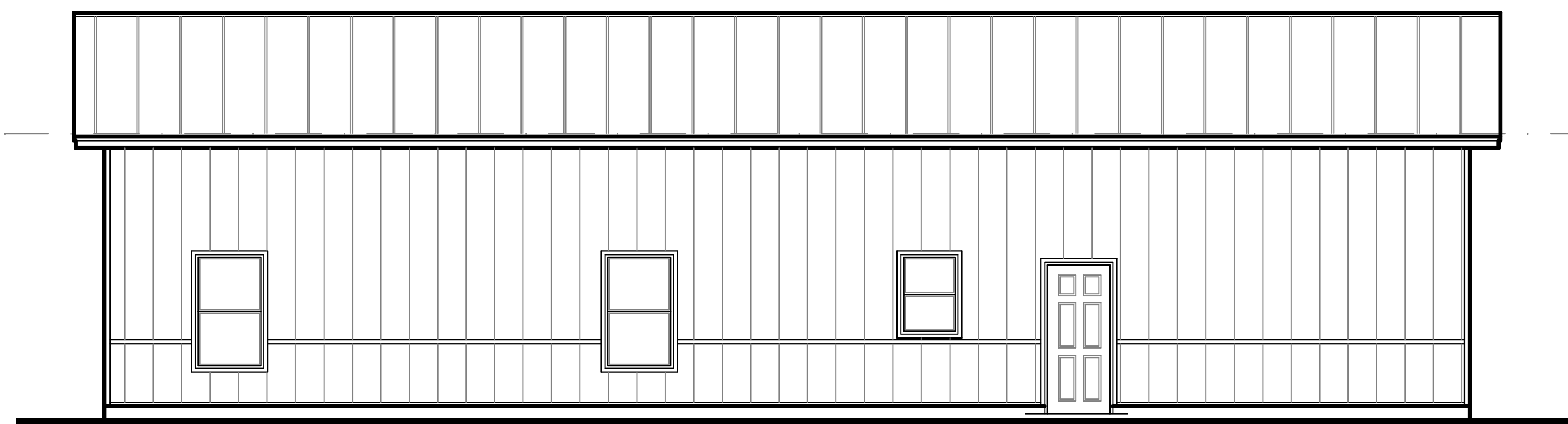
REAR ELEVATION
